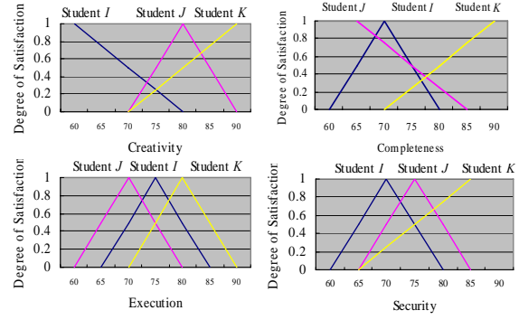
Figure 1. Fuzzy constraints
